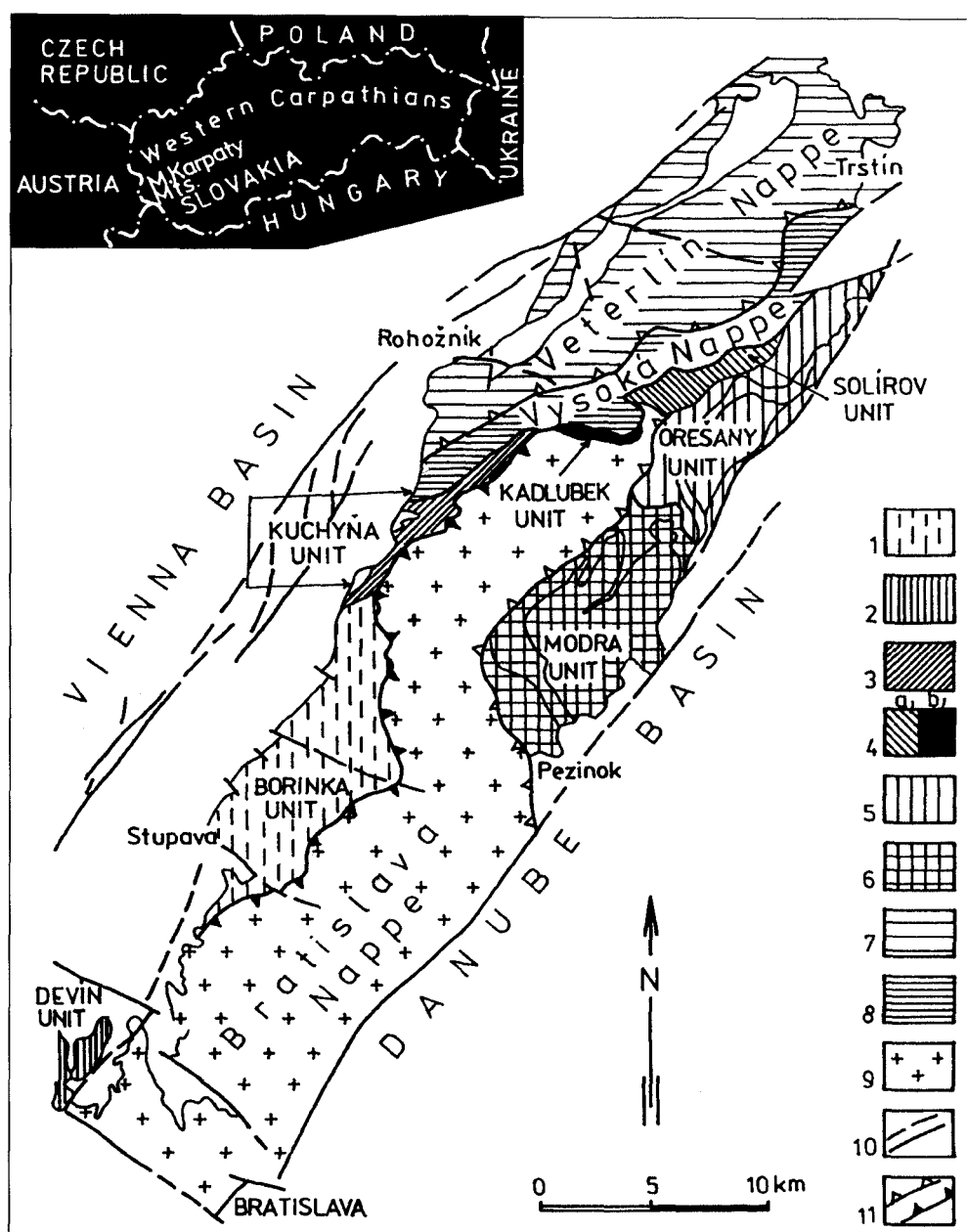
Text-Fig. 1. Tectonic and paleogeographic units of the Malé Karpaty Mts. (after MICHALÍK et al., 1993). 1 = Borinka unit; 2 = Devín unit; 3 = Kuchyňa unit; 4a = Solírov unit; 4b = Kadlubek unit; 5 = Orešany unit; 6 = Modra unit; 7 = Vetrín Nappe; 8 = Vysoká Nappe; 9 = Bratislava Nappe; 10 = faults; 11 = overthrust planes.
