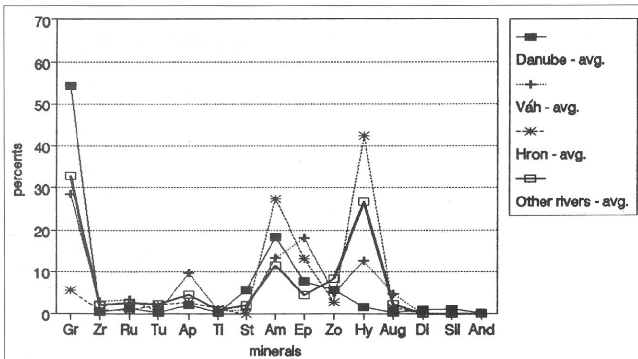
Text-Fig. 16. Graphic representation of heavy minerals contents of the recent Carpathian rivers (after Mišík, 1956). Gr = garnet, Zr = zircon, Ru = rutile, Tu = tourmaline, Ap = apatite, Ti = sphene, St = staurolite, Am = amphibole, Ep = epidote, Zo = zoisite, Hy = hypersthene, Aug = augite, Di = kyanite, Sil = silimanite, And = andalusite.
