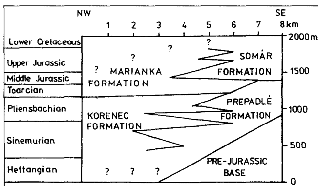
Text-Fig. 2. Facies relations between the formations of the Borinka unit (after PLAŠIENKA, 1987).
