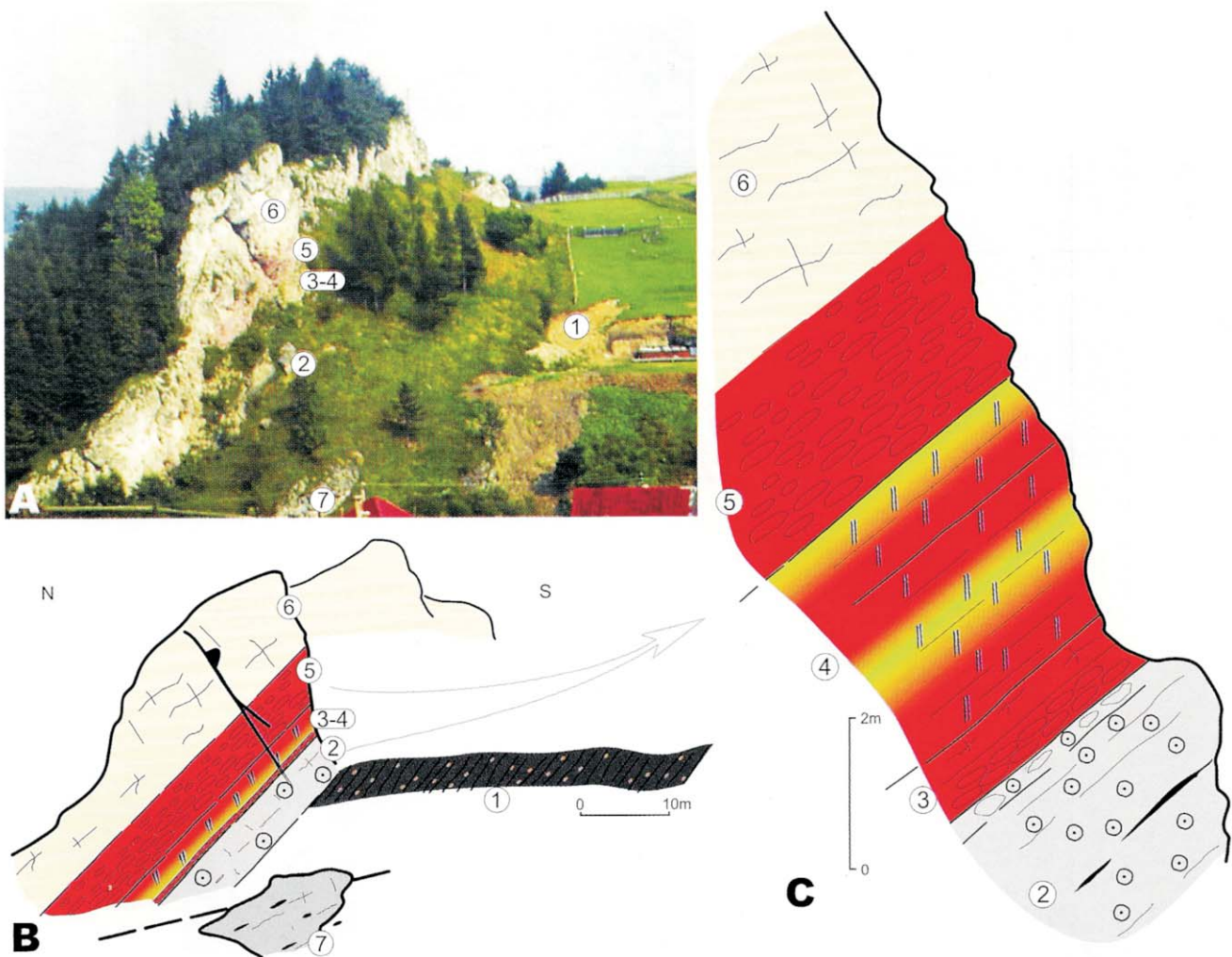
Fig. 6. Litmanovské Klippen section. A–C. General view of the klippen ( A ) and ( B–C ) geological cross-section sketches. Explanations: 1 – black shales with sphaeroidites of the Skrzypny Shale Formation; 2 – grey crinoidal limestones of the Smolegowa Limestone Formation; 3 – ammonitico rosso-type cherry-red nodular limestones of the Niedzica Limestone Formation; 4 – green (lower part) and red (upper part) calcareous radiolarian cherts of the Czajakowa Radiolarite Formation (Podmajerz and Buwałd Radiolarite members, respectively); 5 – ammonitico rosso-type red nodular limestones of the Czorsztyn Limestone Formation; 6 – Calpionella -type white and cream micritic limestones of the Dursztyn Limestone Formation (Sobótka Limestone Member); 7 – maiolica-type grey micritic limestones with cherts of the Pieniny Limestone Formation
