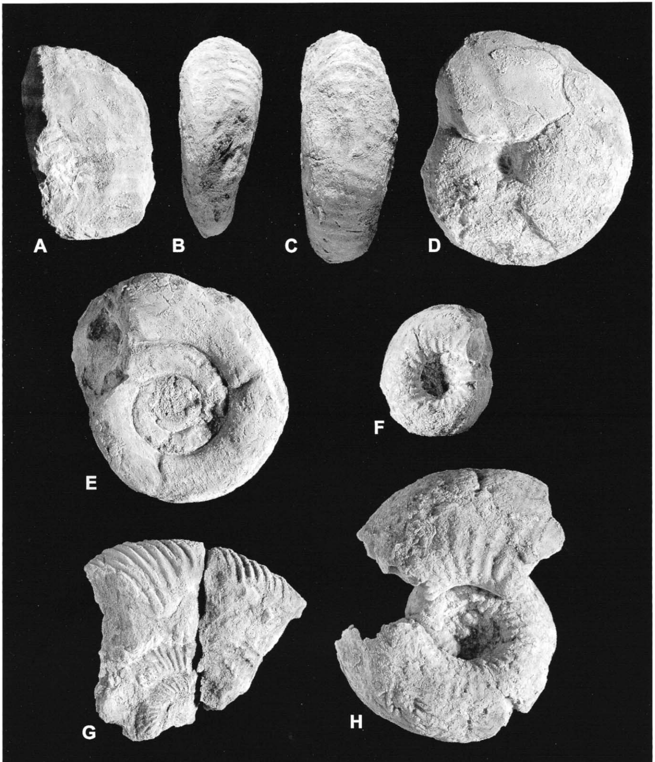
Fig. 8. Ammonites from the Niedzica Limestone Formation of the Czertezik Succession in Milpoš quarry. A–C. Adabofolloceras ex gr. adabofolense (Collignon), 0.1–0.5 m above the base; D. Calliphylloceras disputabile (Zittel), 0.1–0.5 above the base; E. Nannolytoceras tripartitum (Raspail), base of the formation; F. Cadomites ( Cadomites ) cf. daubenyi (Gemmellaro), base of the formation; G. Parkinsonia ( Parkinsonia ) sp., base of the formation; H. Bullatimorphites ( Bullatimorphites ) cf. ymir (Oppel), 1.0–1.1 m above the base, all specimens in natural size; ammonites deposited in Department of Geology and Paleontology of the Comenius University in Bratislava
