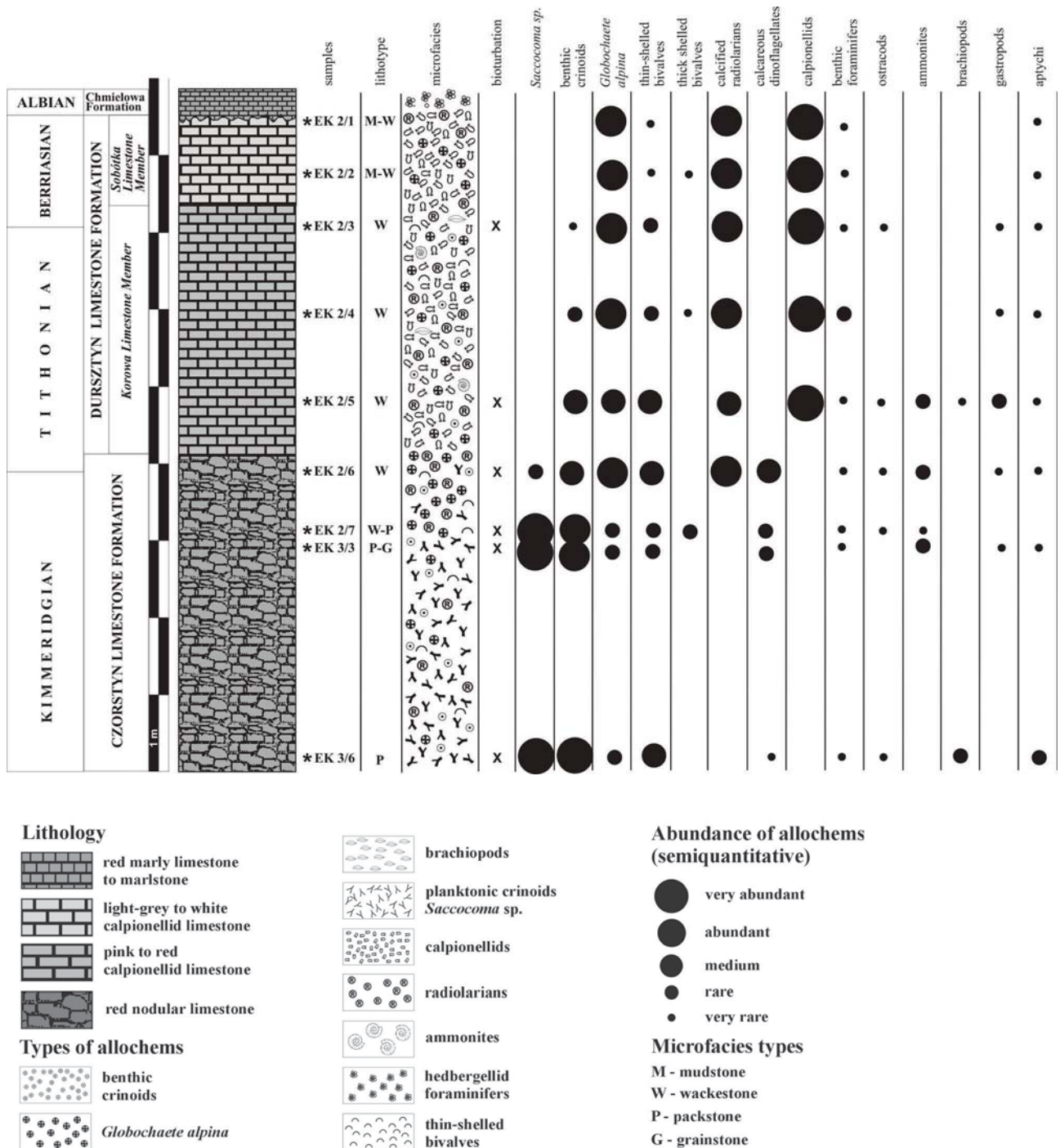
Fig. 3: Lithological section of the examined locality, showing facies and distribution of the allochems.
