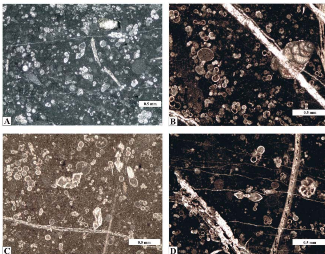
Fig. 12: Planktonic foraminifera and microfossils from the reddish to pink limestones of the Chmielowa Formation from the direct contact with limestones of the Sobótka Limestone Member. A – Foraminiferal and radiolarian wackestone/packstone with Rotalipora cf. appenninica (Renz) and Rotalipora cf. ticinensis (Gandolfi) in the middle. B – Foraminiferal wackestone with Biticinella breggiensis (Gandolfi) (middle left) and Dorothisia sp. (middle right). C – Foraminiferal and radiolarian wackestone with Planomalina buxtoni (Gandolfi). D – Foraminiferal wackestone/packstone with Rotalipora ticinensis (Gandolfi) and Planomalina buxtoni (Gandolfi). All photos from the sample EK2 (see Fig. 10).
