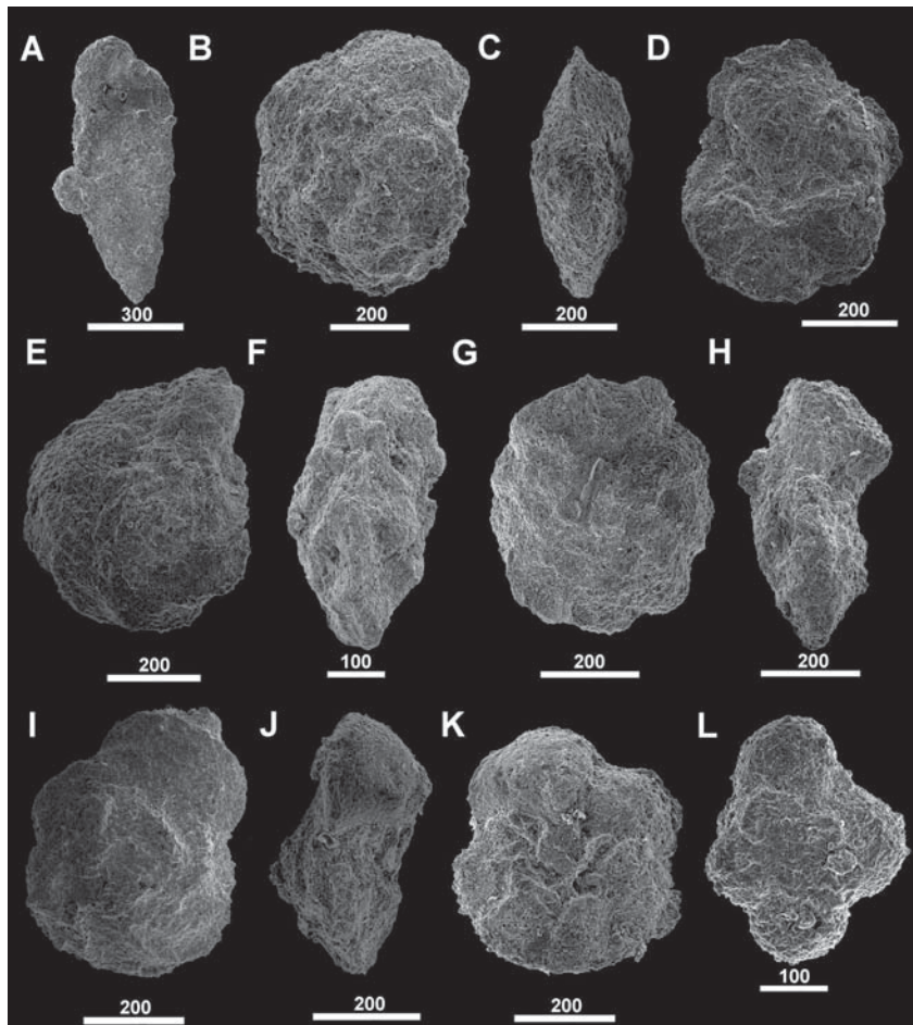
Fig. 11: Foraminifera from the red biodetritic marlstones of the Chmielowa Formation. A – Spiroplectinata complanata Grabert with adherent foraminifer attached to the test. Sample EK4. B–D – Rotalipora appenninica (Renz), B – dorsal, C – peripheral, D – umbilical view. Sample EK1. E–H – Rotalipora ticinensis (Gandolfi), E – dorsal, F,H – peripheral, G – umbilical view. Sample EK4. I–K – Rotalipora globotruncanoides Sigal, I – dorsal, J – peripheral, K – umbilical view. Sample EK1. L – Muricoedbergella simplex (Morrow), dorsal view. Sample EK4. For sample numbers see Fig. 10. Scale is in microns.
